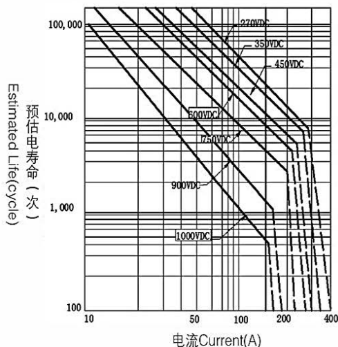
1. 阻性负载下产品通、断电寿命预估次数曲线 Product life estimated (make/break) curve under resistive load
